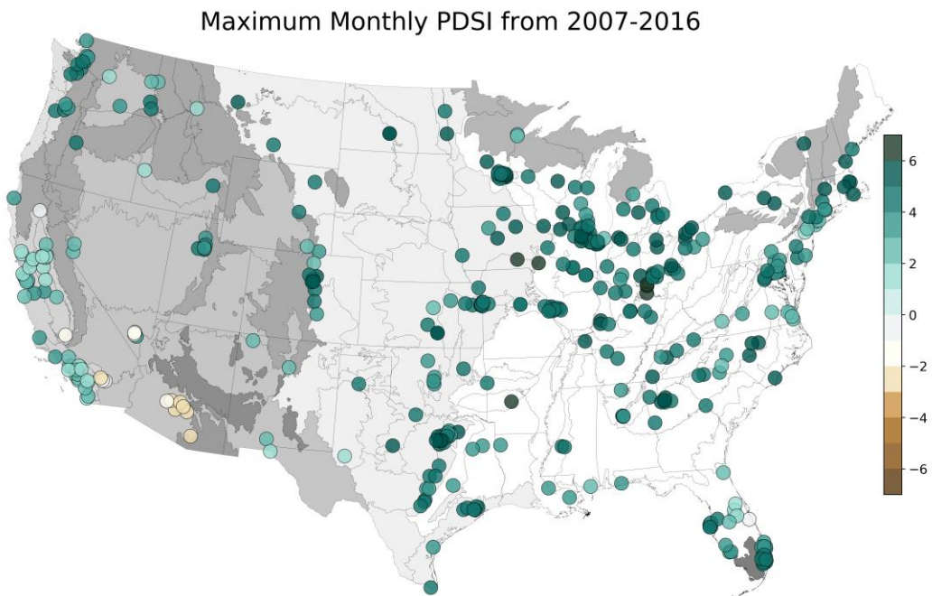
Figure 2. Monthly extremes of low soil moisture (minimum PDSI; Palmer Drought Severity Index) and high soil moisture (maximum PDSI) for the most recent ten-year period (2007-2016) at sampled Parks and Recreation Department locations.
